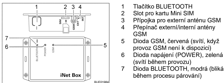
Obr. 140 Truma iNet-Box
