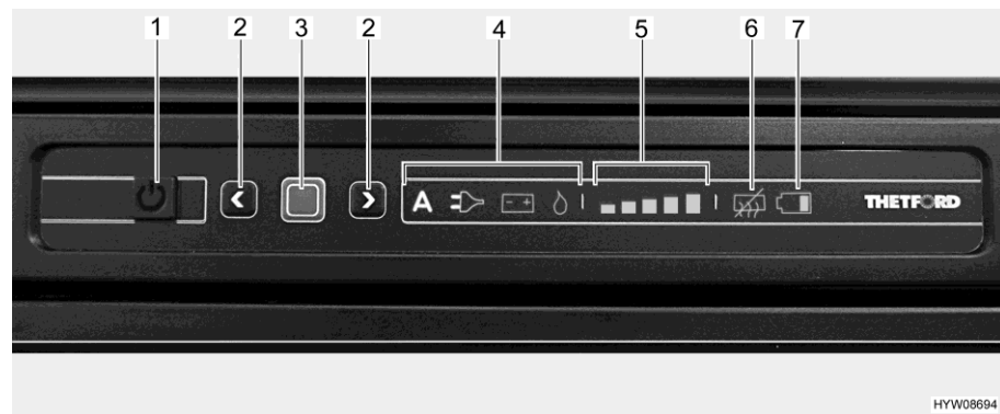
Afb. 195 LED-bedieningsveld (Thetford-koelkast)
