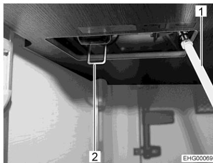
Afb. 108 Handslinger in garage achter
