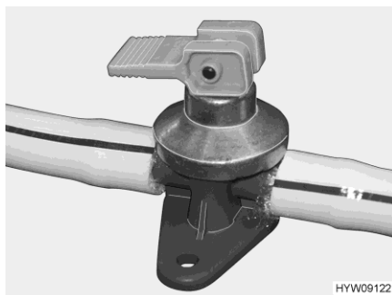
Afb. 166 Aftapkraan (boiler Alde)
